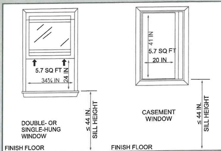
Figure 3 Single- or double-hung or casement window
