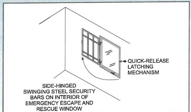
Figure 10 Security bars
